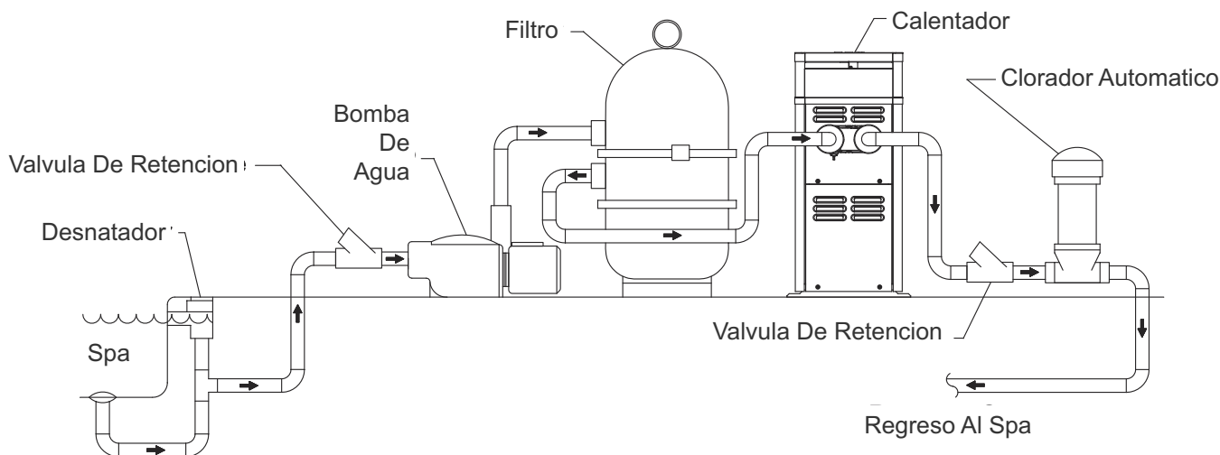
Fig. 1: Spa/Chlorinator Setup
